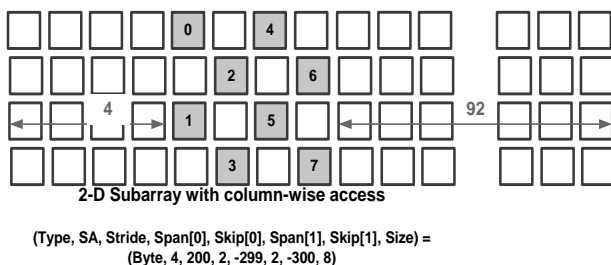
Figure 1. Stream descriptors for a memory access pattern
