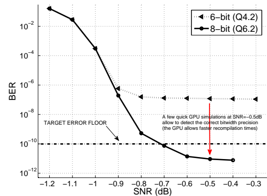
Figure 8: BER curves simulation for 6- and 8-bit variable width precision for a given target error floor.
