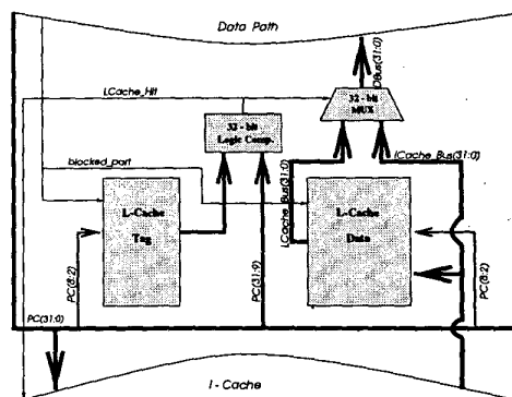
Figure 3: L-Cache organization
