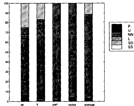
Figure 4: Instruction placement results for the SPECint95 benchmarks with a 0.5KB L-Cache
